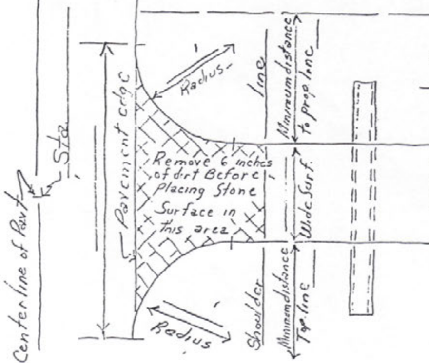
PLAN VIEW OF ENTRANCE
